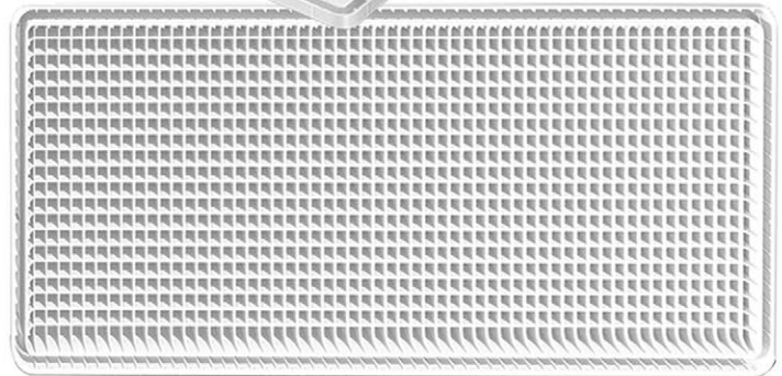
(above) The Maximus lid cell structure is engineered for superior strength (below) Deep set tongue-in-groove closure
